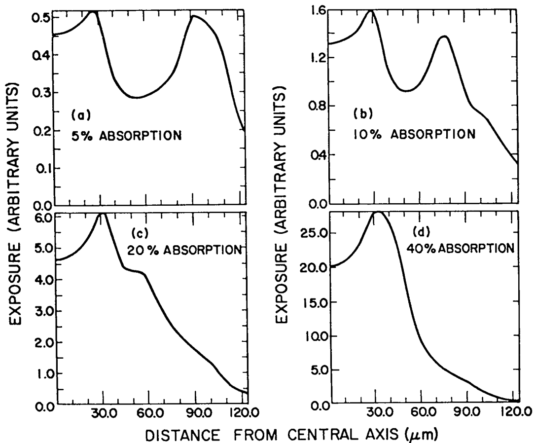
Fig. III-7. Theoretical prediction of soft x-ray pinhole pictures (10- \mu m resolution).
