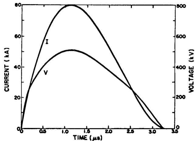
Fig. II-5. Calculated voltage and current waveforms for prototype power amplifier.
