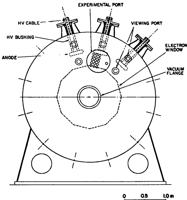
Fig. II-2. End view of Antares prototype power amplifier.
