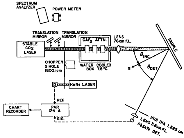
Fig. II-3. Schematic of experimental setup for measuring surface reflection coefficients at 10 \mu m.
